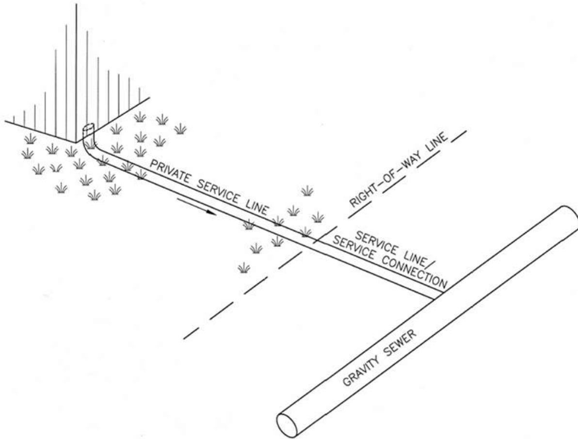
TYPICAL GRAVITY SEWER SCHEMATIC
