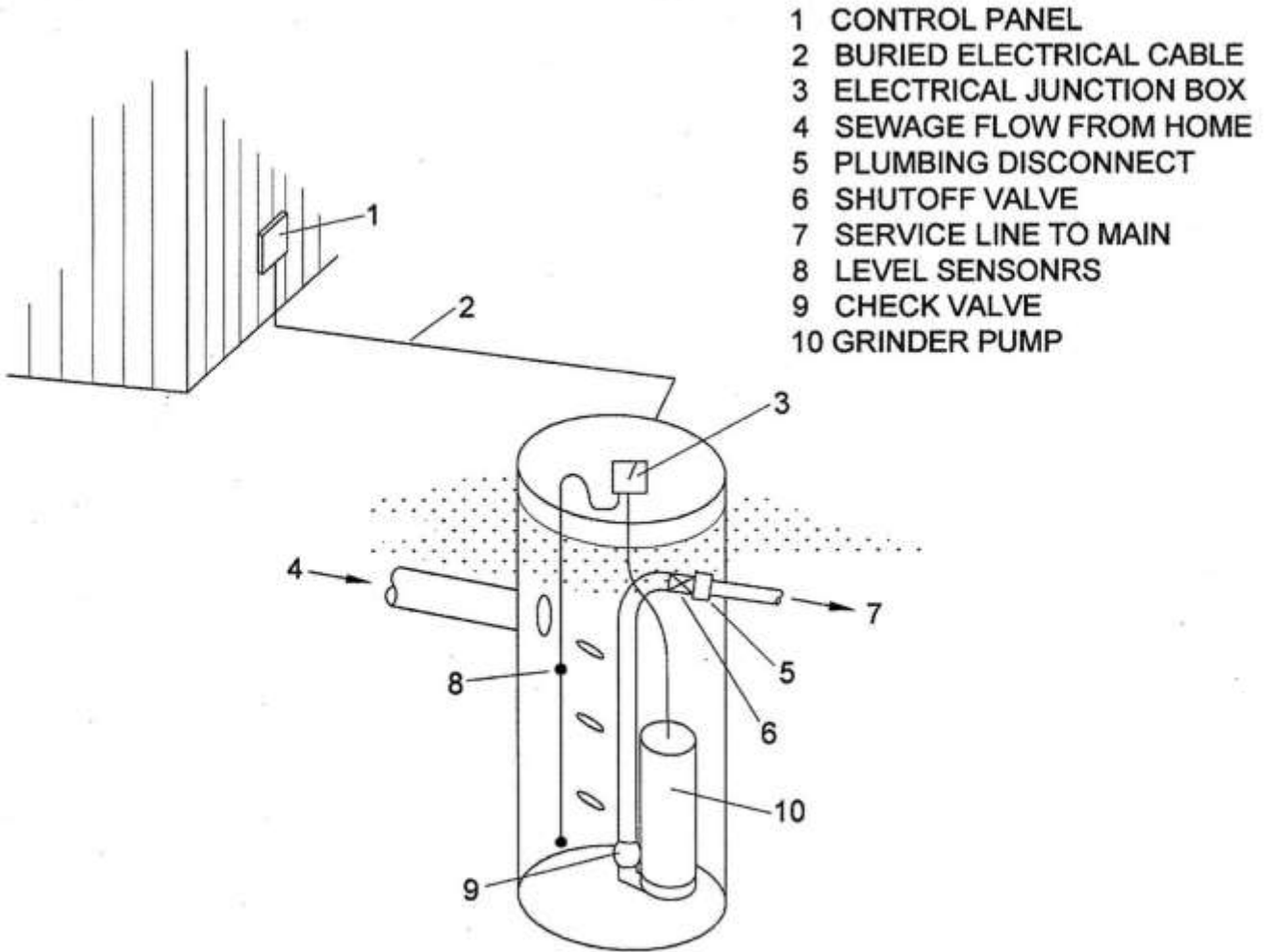
TYPICAL GRINDER PUMP PRESSURE SEWER SCHEMATIC
